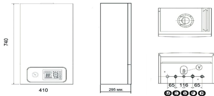
Gas boiler connect size and installation map 产品接口尺寸及安装示意图
